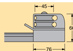
MOD. 4274G End fitting, 2 sheaves (D = 45 mm) and becket
