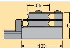
MOD. 4274Z End fitting, 2 sheaves (D = 55 mm) and becket
