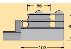
MOD. 4274Z End fitting, 2 sheaves (D = 55 mm) and becket
