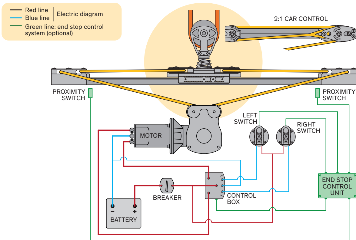
SWITCHES
