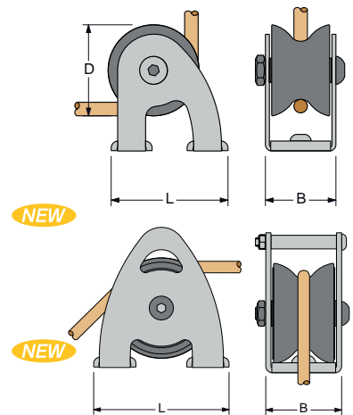
MOD. 818.050 - OVER THE TOP
