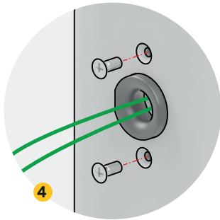
4 Put the Fairlead into place using the line, fit the screws, take off the line and tighten screws.
